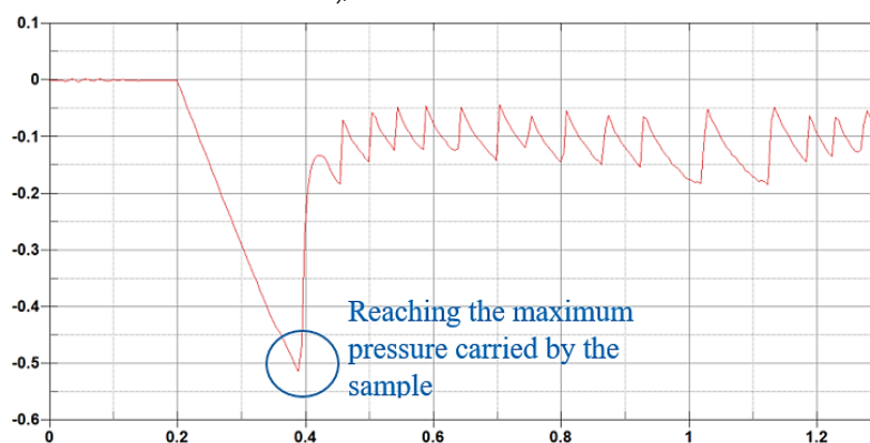
Fig. 4. Values of reaction force RY [N] as a function of time [s] in one of the vertical constraints of the lower pressure plate
